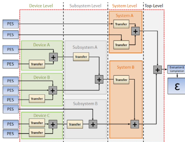
Figure 9. Proper grouping of subsystems
