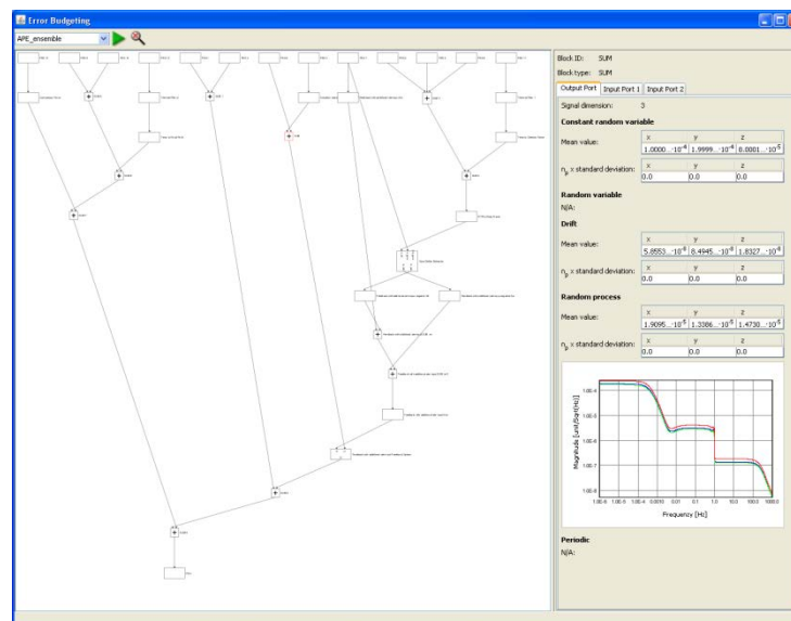
Figure 7. Tree View
