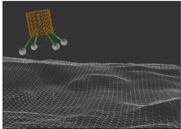
Contact dynamics for landing simulations
